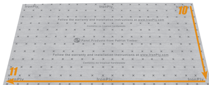
Fastener Diagram 10, 11
